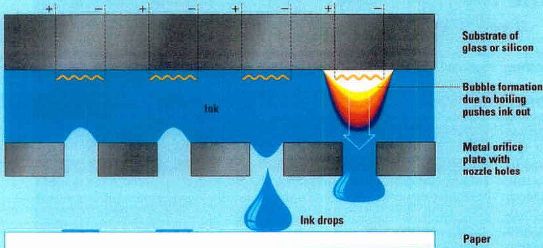
Electric current heats resistors, causing ink to boil and spit out.
